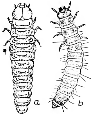
Fig. 23. a, Caraboid instar of meloid larva; b, saw-toothed grain beetle, Oryzaephilus surinamensis (L.)
